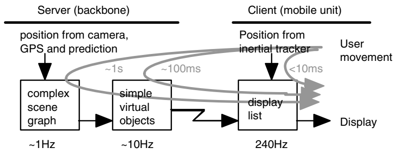
Figure 2. Latency layered rendering system.
