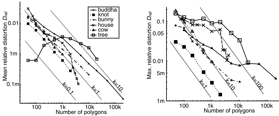
Figure 5. Mean and maximum relative distortion. Cow from [QSlim99]. Tree and House (Maybeck Studio) from [Artifice99]. Buddha and Bunny From [Stanford96]. Knot is a pipe bent into a 3-dimensional lissajour figure.
