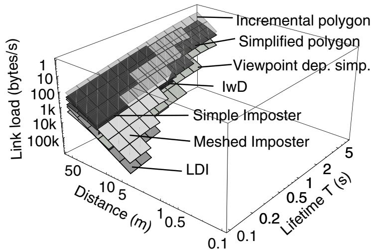
Figure 12. As Figure 11, but now the number of polygons N is limited to 500.
