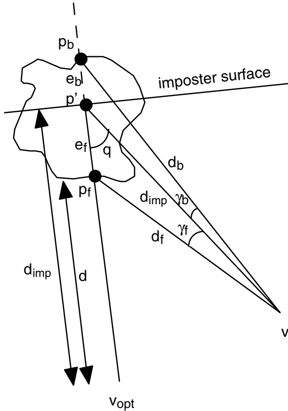
Figure 7. Visual distortion \gamma caused by movement of viewpoint away from the optimal viewpoint.
