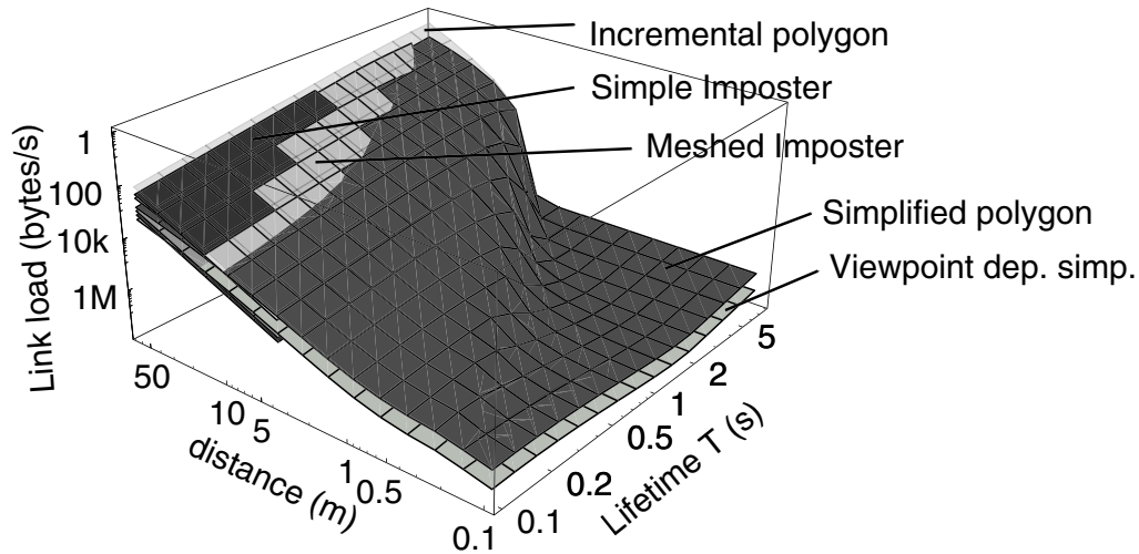
Figure 11. Average load on the communication link. Maximum distortion D=0.001 , and object size r=1 m. Incrementally transported simplified polygon objects are shown transparent to expose underlying layers.
