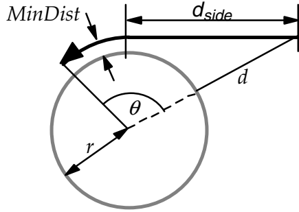
Figure 9. Maximum angular distance the observer can walk around the object \theta . Thick black: the walking path. Thick grey: boundary of the object.
