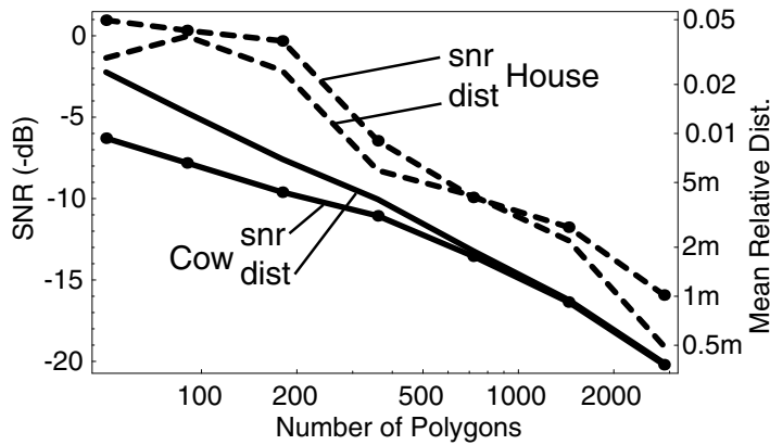
Figure 15. Comparison of mean relative distortion and SNR. Vertical placement of SNR and dist curves is arbitrary, chosen such that right sides of the cow curves match.
