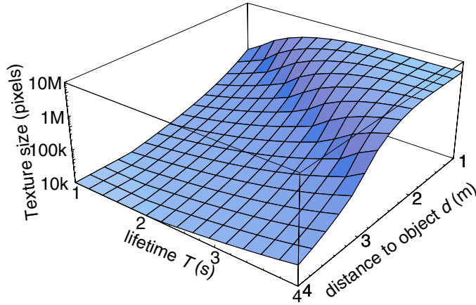
Figure 10. Uncompressed texture size as a function of the lifetime T and the distance to the object d . Distortion D=0.004 rad, object size r=0.5 m, v=0.7 m/s and MinDist=0.2 m.
